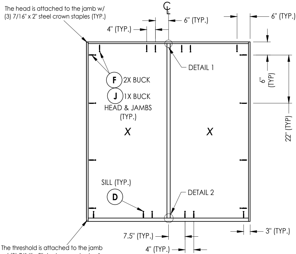
FRAME ANCHORING
