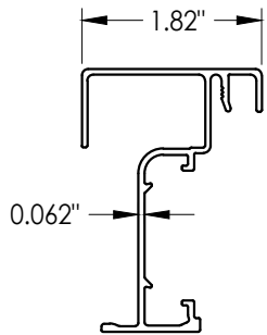
"MODERN" PROFILE
