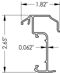
"TRADITIONAL" PROFILE
